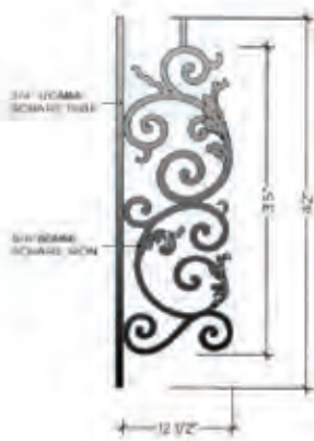
TOP VIEW A-2 ALL RADIUS FROM 20" TO 200" HFBX.A2
